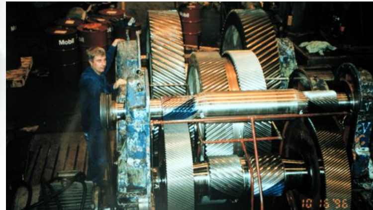
Modernization of a gearbox for cement kiln
